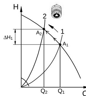
Fig. 7 Uncontrolled pump
