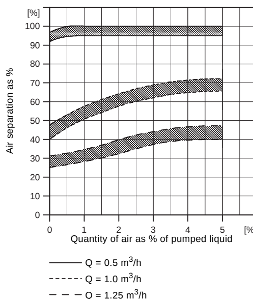
Fig. 14 Air separation
