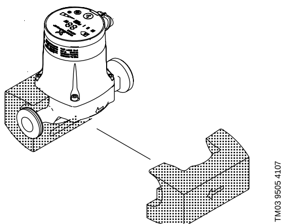
Fig. 18 Insulating shells
